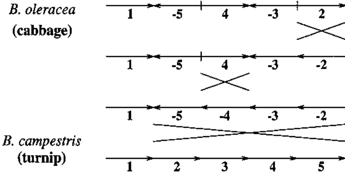
Figure 10.1: "Transformation" of cabbage into turnip.
