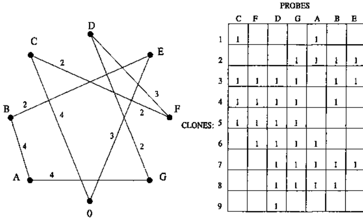
Figure 3.1: Shortest cycle for the Hamming Distance TSP corresponding to the hybridization matrix in Figure 1.1 with a different order of columns. The shown minimum cycle defines the ordering of clones with the minimum number of gaps. Clones 1, 3, and 4 in this ordering are chimeric.
