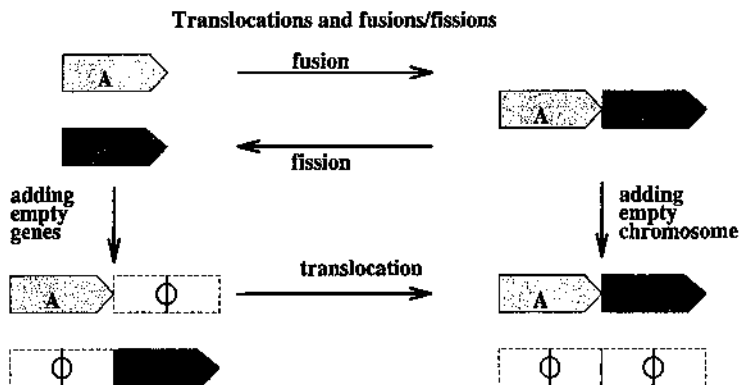
Figure 10.18: Fusions/fissions can be mimicked by translocations by introducing empty chromosomes.
