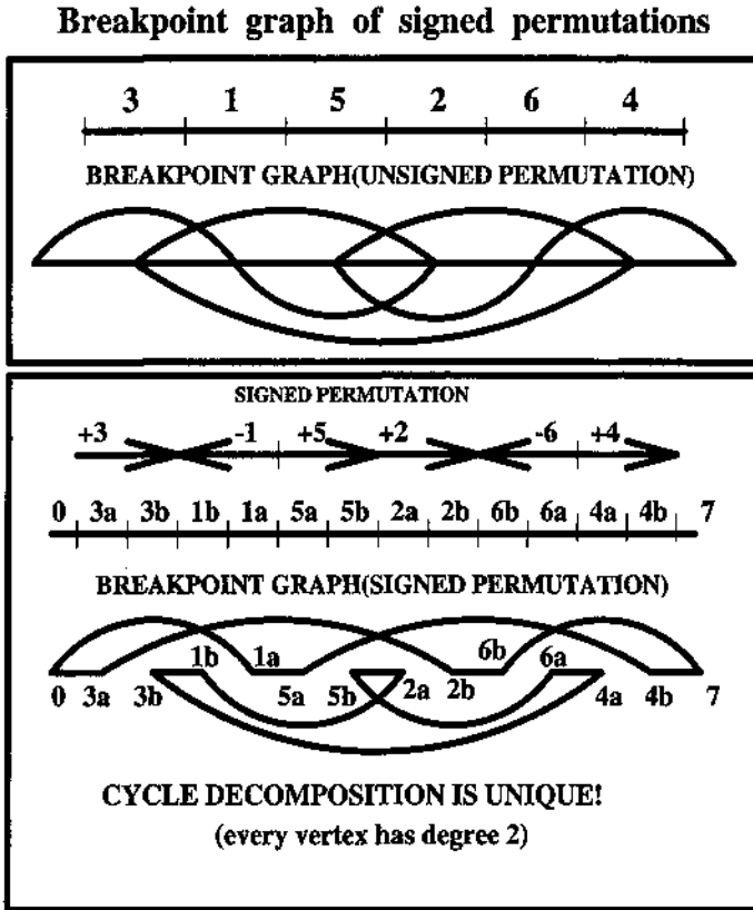
Figure 10.5: Modeling a signed permutation by an unsigned permutation.
