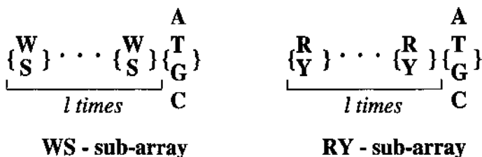
Figure 5.11: Binary arrays.
