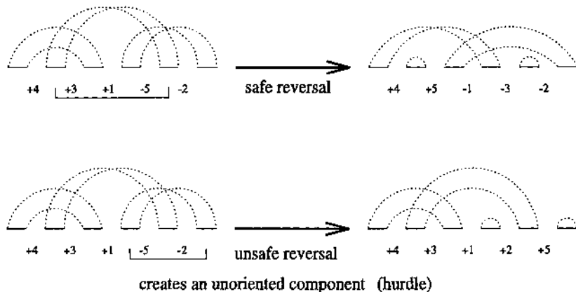
Figure 10.14: Examples of safe and unsafe reversals.
