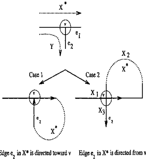
Figure 2.9: Two cases in theorem 2.
