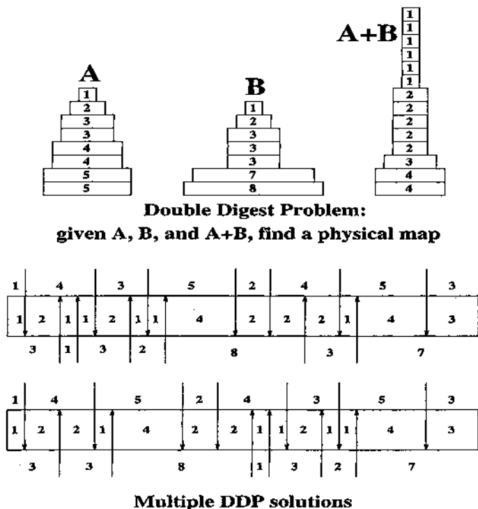
Figure 2.3: The Double Digest Problem may have multiple solutions.
