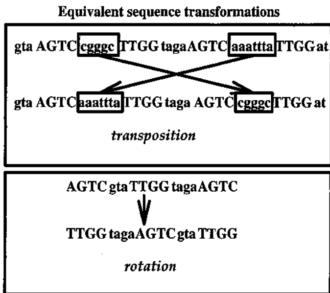
Figure 5.9: Ukkonen's transformations ( l = 5 ).
