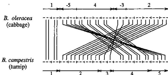
Figure 10.6: Comparative physical map of cabbage and turnip (unsigned permutation) and corresponding signed permutation.
