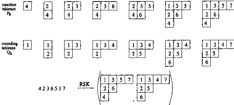
Figure 6.5: RSK algorithm for permutation \pi = 4236517 .
