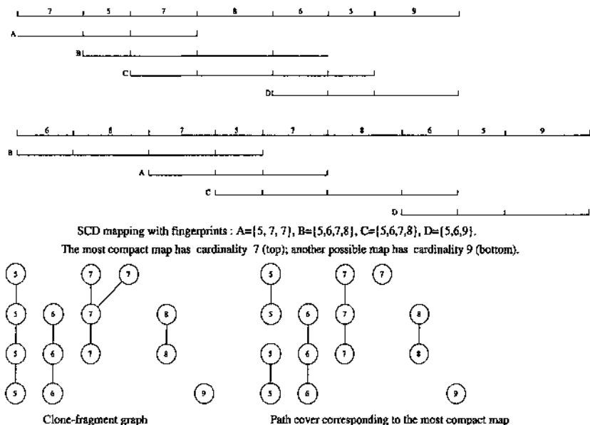
Figure 3.6: SCD mapping.
