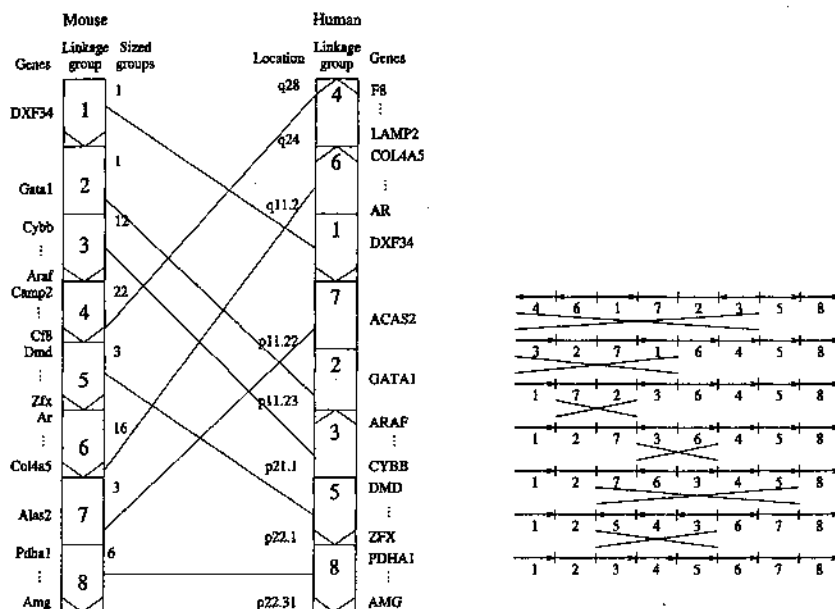
Figure 1.5: "Transformation" of a human X chromosome into a mouse X chromosome.
