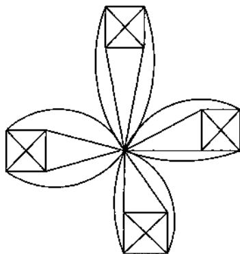
Figure 7.1: 5-star with four cliques.
