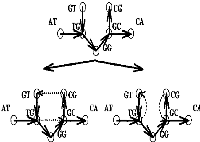
Figure 5.7: Sequence reconstruction in the case of missing l -tuples (false negative).
