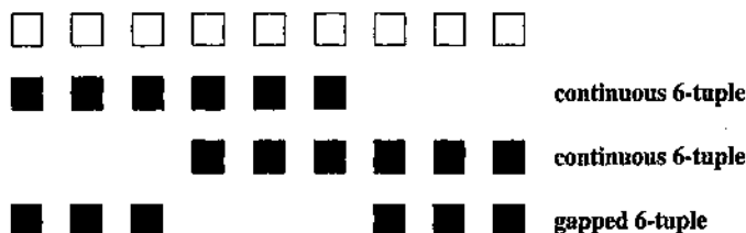
Figure 6.8: Every 9-match with one error contains either a continuous 6-match or a gapped 6-match.
