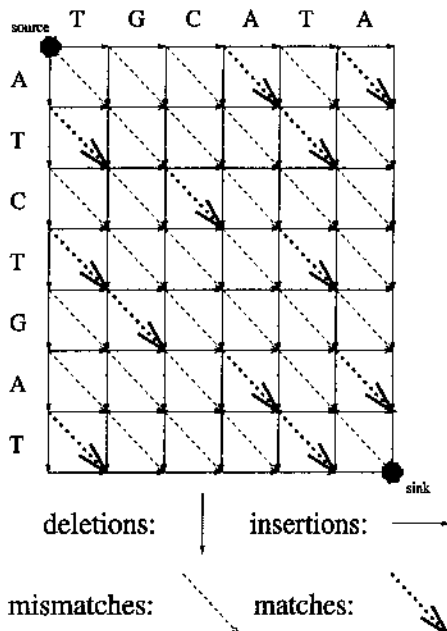
Figure 6.2: Edit graph. The weights of insertion and deletion edges are -\sigma , the weights of mismatch edges are -\mu , and the weights of match edges are 1.
