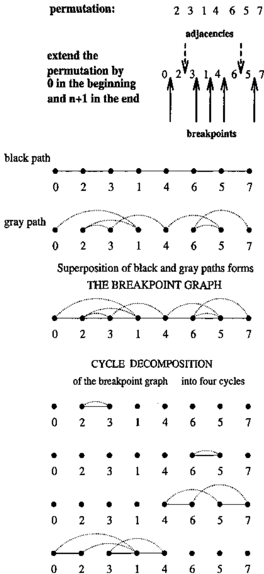
Figure 10.4: Breakpoints, breakpoint graph, and maximum cycle decomposition.
