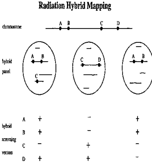
Figure 3.7: Hybrid screening matrix.
