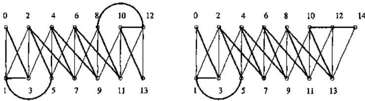
Figure 10.8: G(\gamma_{12}) and G(\gamma_{13}) .
