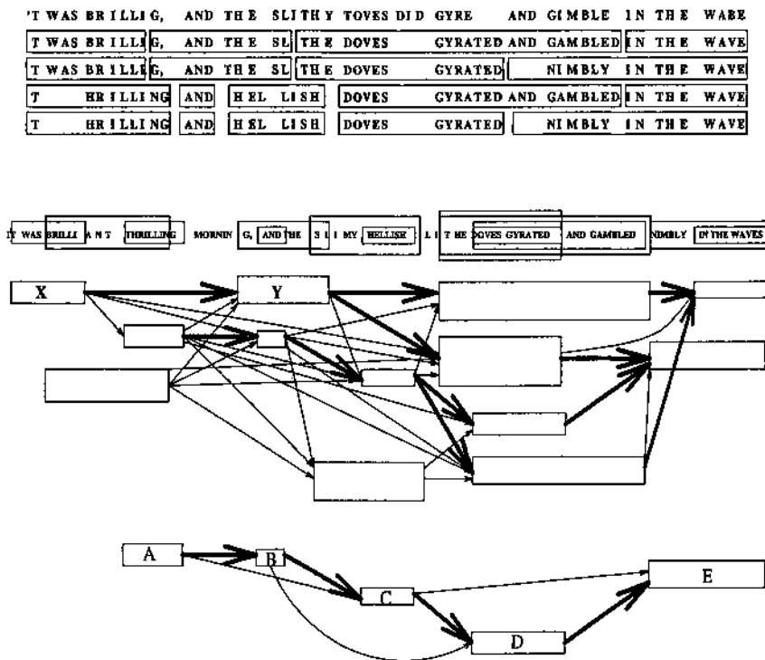
Figure 9.11: Constructing an Alternative Splicing Encyclopedia (ASE) from potential exons. Four different splicing variants (above) correspond to four paths (shown by bold edges) in the exon assembly graph. The overall number of paths in this graph is large, and the problem is how to identify paths that correspond to real splicing variants. The graph at the bottom represents the trimmed exon assembly graph with just five potential splicing variants (paths).
