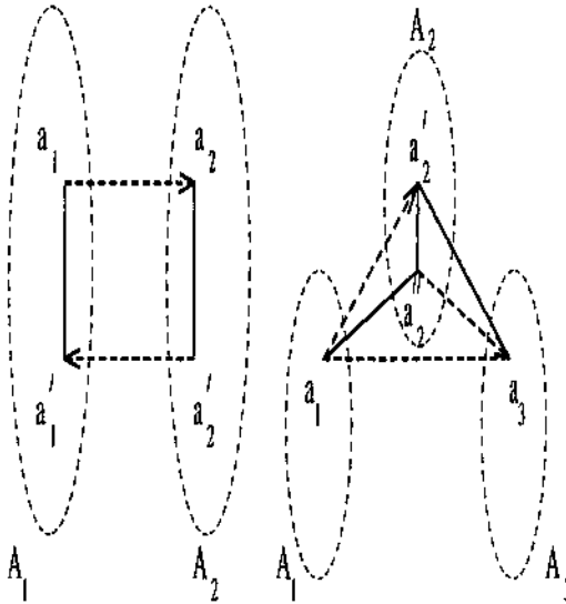
Figure 3.5: Proof of theorem 3.1.
