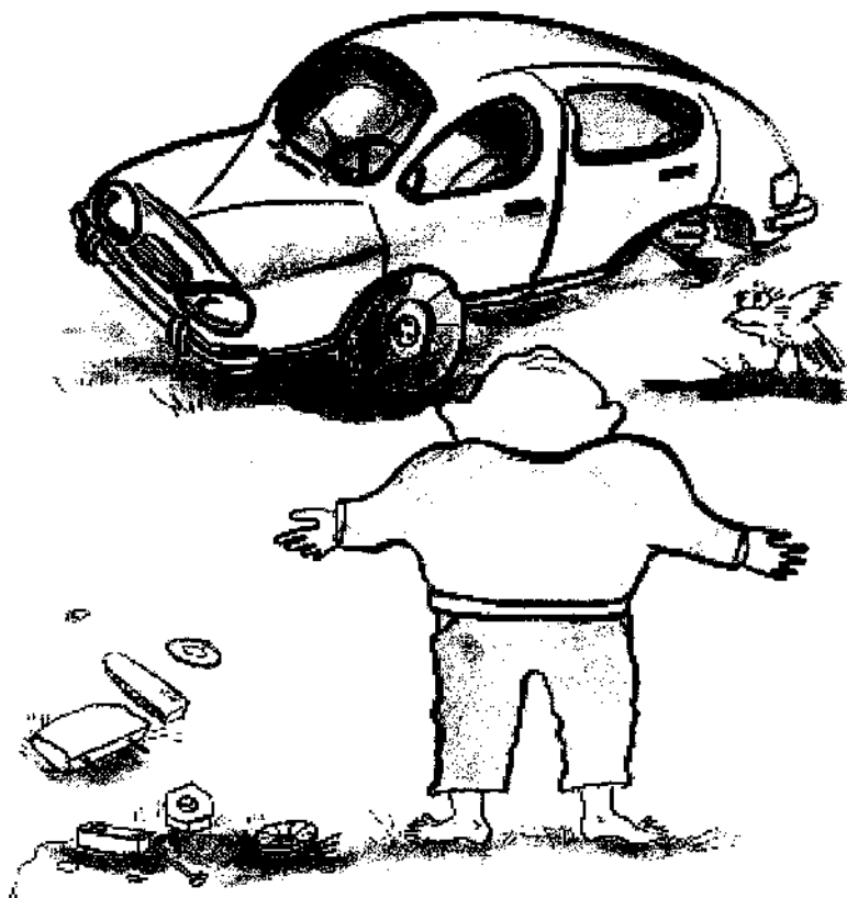
Figure 9.7: And assembling...
