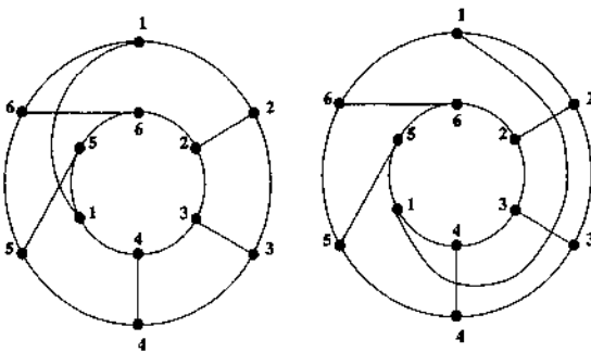
Figure 12.2: Crossing edges in embeddings.
