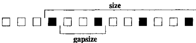
Gapped 4-tuple with gapsize 3 and size 10 starting at position 4
