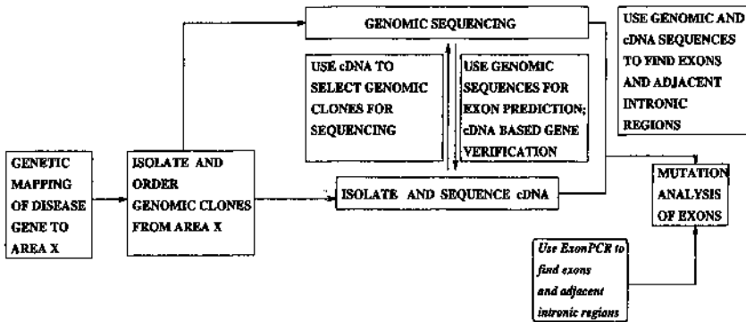
Figure 9.10: Positional cloning and ExonPCR.
