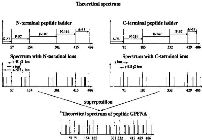
Figure 11.1: Theoretical MS/MS spectrum of peptide GPFNA with parent mass 57 + 97 + 147 + 114 + 71 = 486 .
