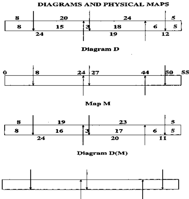
Figure 12.1: Diagrams and physical maps.
