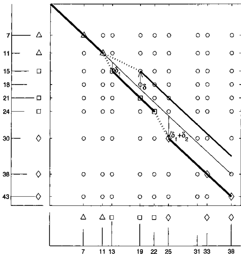
Figure 11.8: Aligning spectra. The shared peaks count reveals only D(0) = 3 matching peaks on the main diagonal, while spectral alignment reveals more hidden similarities between spectra ( D(1) = 5 and D(2) = 8 ) and detects the corresponding mutations.
