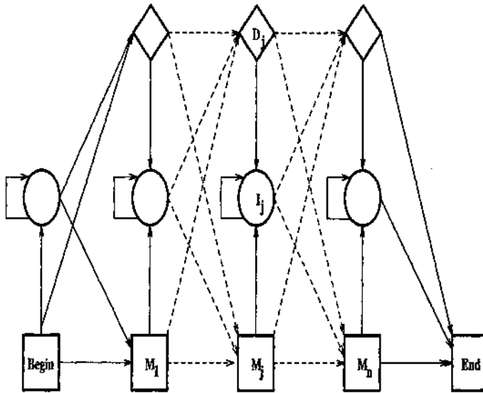
Figure 8.3: Profile HMM.
