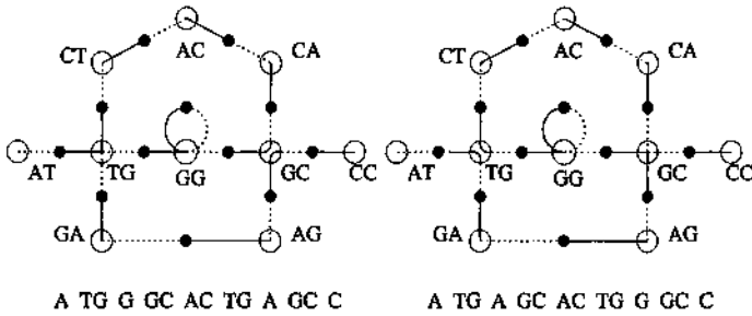
Figure 5.10: Ukkonen's conjecture. The sequence (Eulerian path) on the right is obtained from the sequence on the left by a transposition defined by the interleaving pairs of dinucleotides TG and GC.
