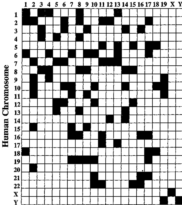
Figure 1.4: Man-mouse comparative physical map.
