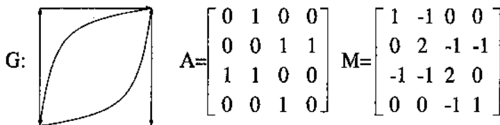
Figure 5.6: Each cofactor of the matrix M is 2. The number of Eulerian cycles in graph G is 2 \cdot 0! \cdot 1! \cdot 1! \cdot 0! = 2 .
