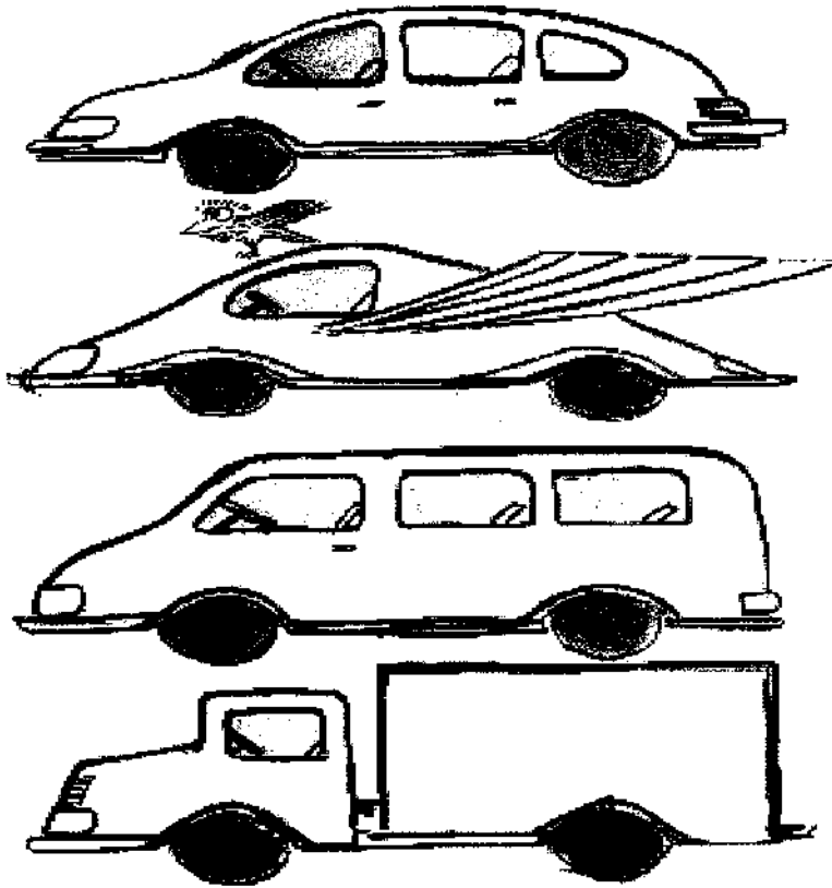
Figure 9.9: Selecting the best exon assembly.
