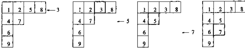
Figure 6.4: Row insertion of 3 into Young tableaux.
