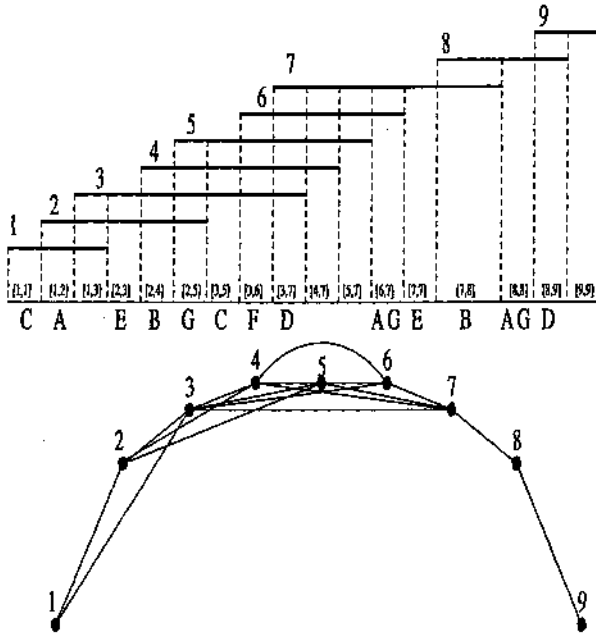
Figure 3.2: Atomic intervals.
