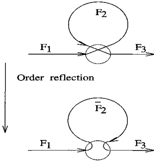
Figure 2.8: Order reflection.
