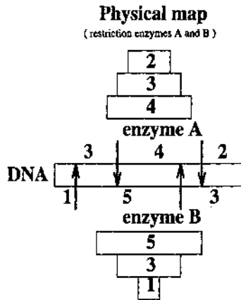
Figure 2.1: Physical map of two restriction enzymes. Gel-electrophoresis provides information about the sizes (but not the order) of restriction fragments.
