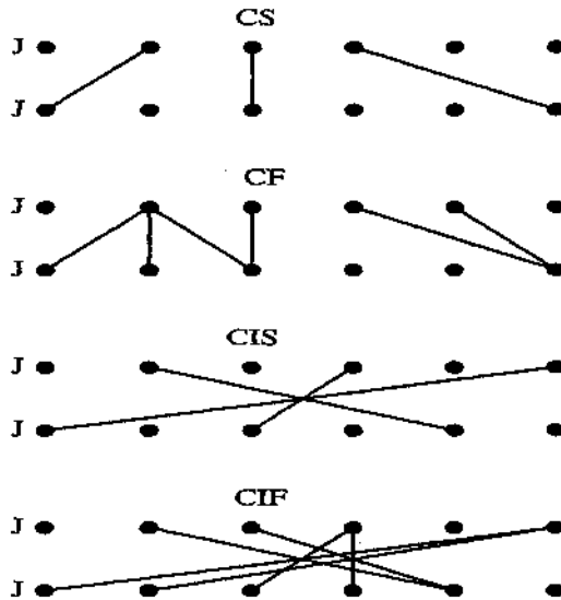
Figure 6.6: Chains in partial orders CS, CF, CIS, and CIF.
