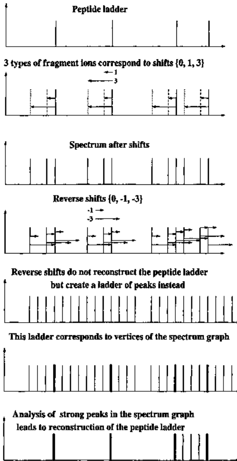
Figure 11.3: Reverse shifts create a set of vertices in the spectrum graph. “Strong peaks” (shown by solid bars) correspond to peaks that are obtained by multiple reverse shifts.
