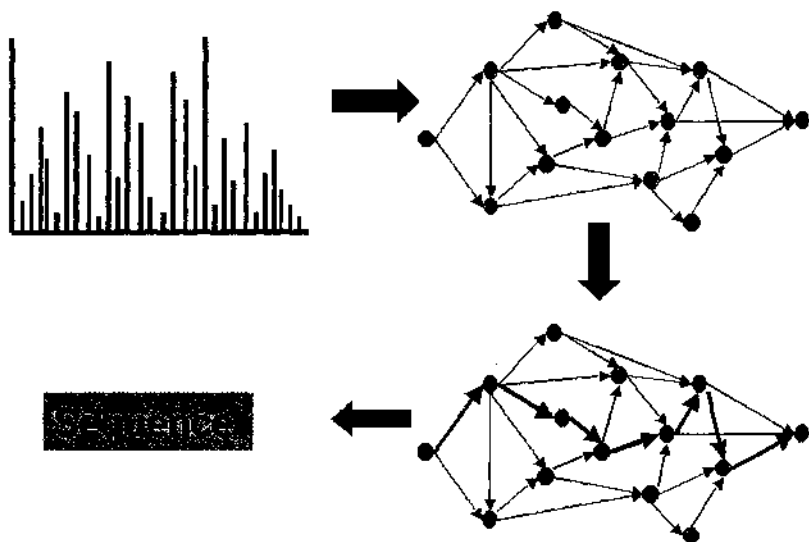
Figure 11.5: Noise in a spectrum generates many “false” edges and vertices in the spectrum graph and disguises edges corresponding to the real peptide sequence. Sequence reconstruction corresponds to finding an optimal path in the spectrum graph.
