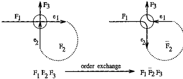
Figure 2.10: Case 1: Order exchange.
