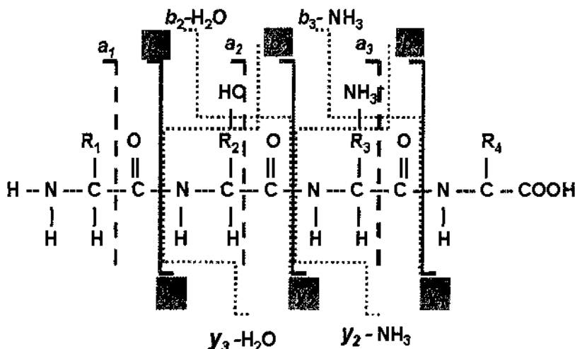
Figure 11.2: Typical fragmentation patterns in tandem mass spectrometry.
