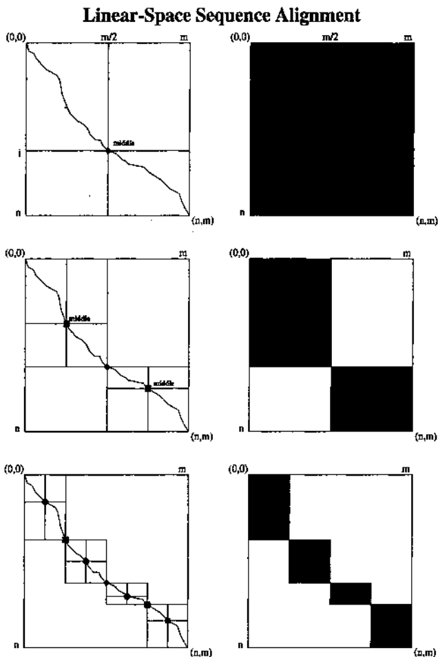
Figure 6.3: Space-efficient sequence alignment. The computational time (area of solid rectangles) decreases by a factor of 2 at every iteration.
