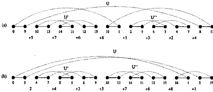
Figure 10.11: (a) Unoriented component U separates U' and U'' by virtue of the edge (0, 1) ; (b) Hurdle U does not separate U' and U'' .
