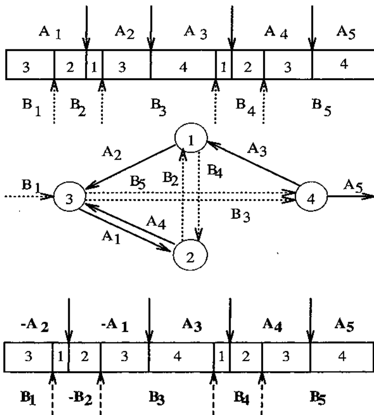
Figure 2.12: Fork graph of a physical map with added extra edges B_1 and A_5 . Solid (dotted) edges correspond to multiforks of A ( B ). Arrows on the edges of this (undirected) graph follow the path B_1 A_1 B_2 A_2 B_3 A_3 B_4 A_4 B_5 A_5 , corresponding to the map at the top. A map at the bottom B_1 - A_2 - B_2 - A_1 B_3 A_3 B_4 A_4 B_5 A_5 is obtained by changing the direction of edges in the triangle A_1, B_2, A_2 (cassette reflection).
