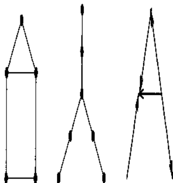
Figure 3.4: (i) The house graph is not an interval graph because it is not triangulated. (ii) The star graph is not an interval graph because its complement is not a comparability graph. (iii) Transitive orientation of a graph "A."
