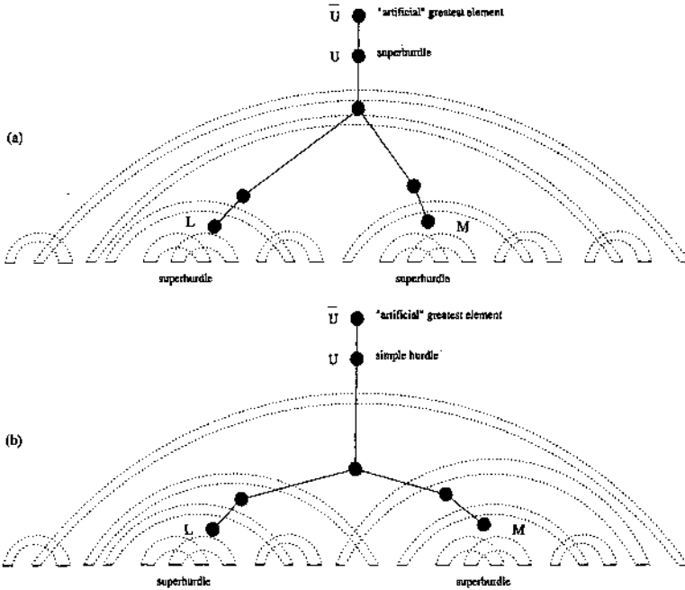
Figure 10.16: The permutation in (a) is a 3-fortress, while the permutation in (b), with the same cover graph, is not a fortress (hurdle U is not a superhurdle).
