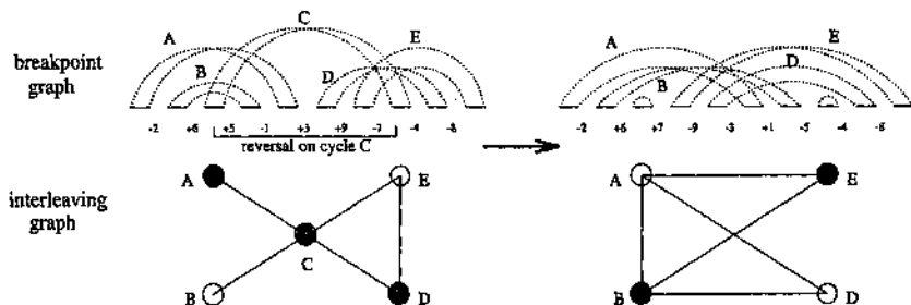
Figure 10.13: Reversal on a cycle C complements the edges between the neighbors of C and changes the orientation of each cycle neighboring C in the interleaving graph.
