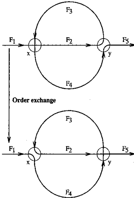
Figure 2.7: Order exchange.
