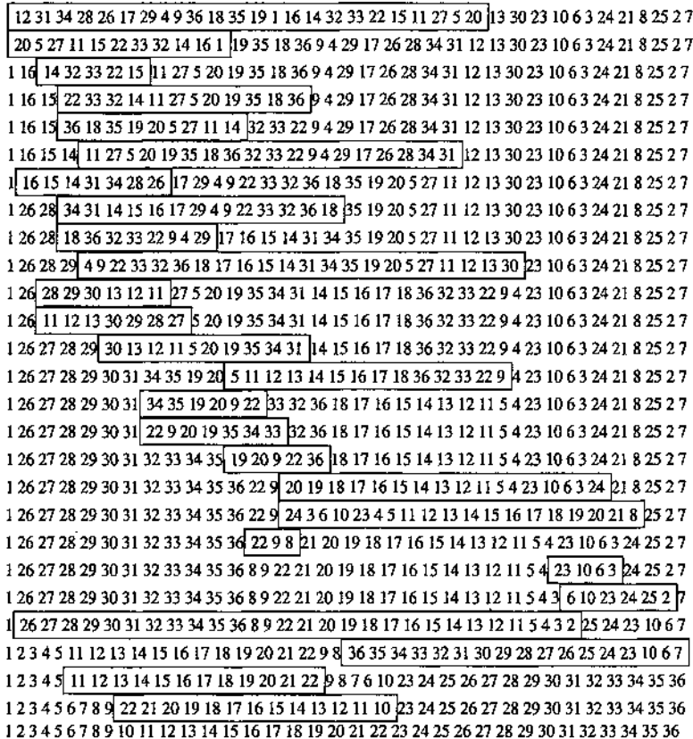
Figure 10.2: A most parsimonious rearrangement scenario for transformation of worm Ascaris Suum mitochondrial DNA into human mitochondrial DNA (26 reversals).
