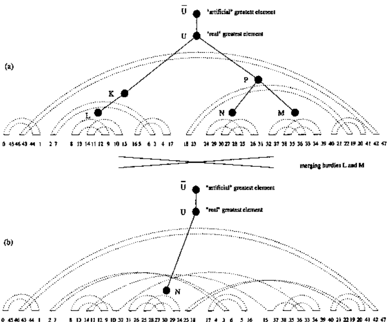
Figure 10.15: (a) A cover graph \Omega_\pi of a permutation \pi with “real” unoriented components K, L, M, N, P , and U and an “artificial” component \bar{U} ; (b) A reversal \rho merging hurdles L and M in \pi transforms unoriented components L, K, P , and M into an oriented component that “disappears” from \Omega_{\pi\rho} . This reversal transforms unoriented cycles (32, 33, 36, 37, 32) and (10, 11, 14, 15, 10) in \pi into an oriented cycle (15, 14, 11, 10, 32, 33, 36, 37, 15) in \pi\rho . LCA(L, M) = \overline{LCA}(L, M) = U and PATH(A, F) = \{L, K, U, P, M\} .
