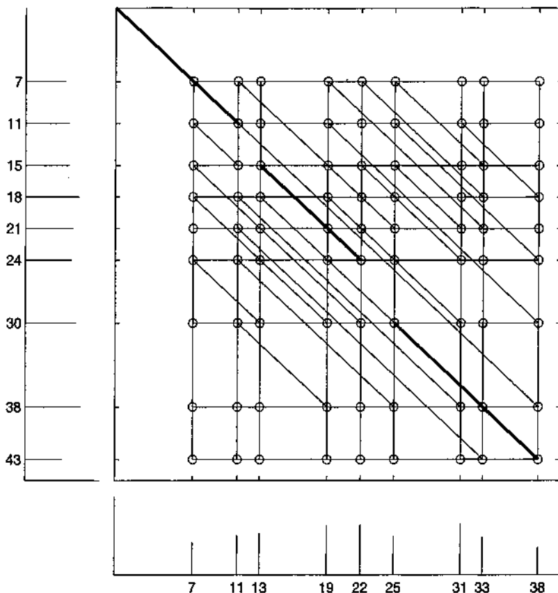
Figure 11.9: Modification of a dynamic programming graph leads to a fast spectral alignment algorithm.
