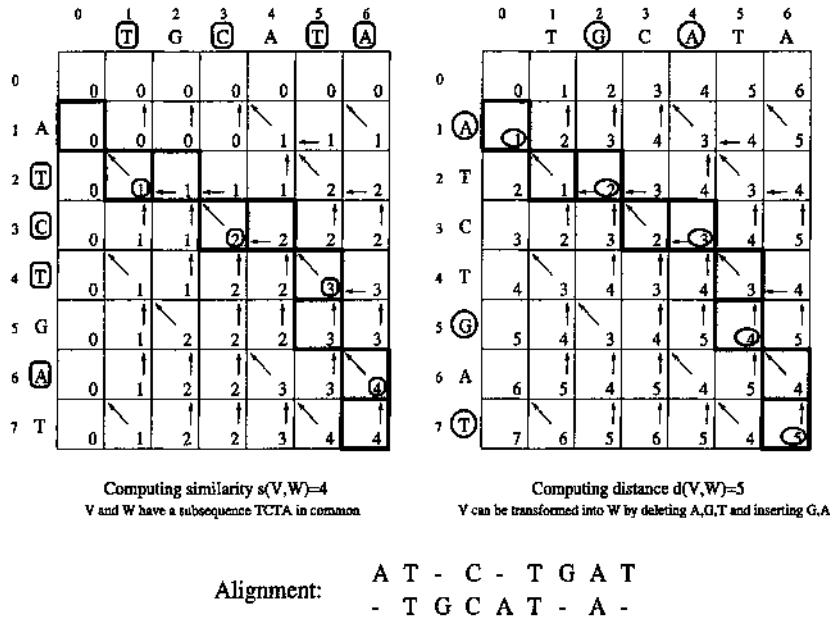
Figure 6.1: Dynamic programming algorithm for computing longest common subsequence.
